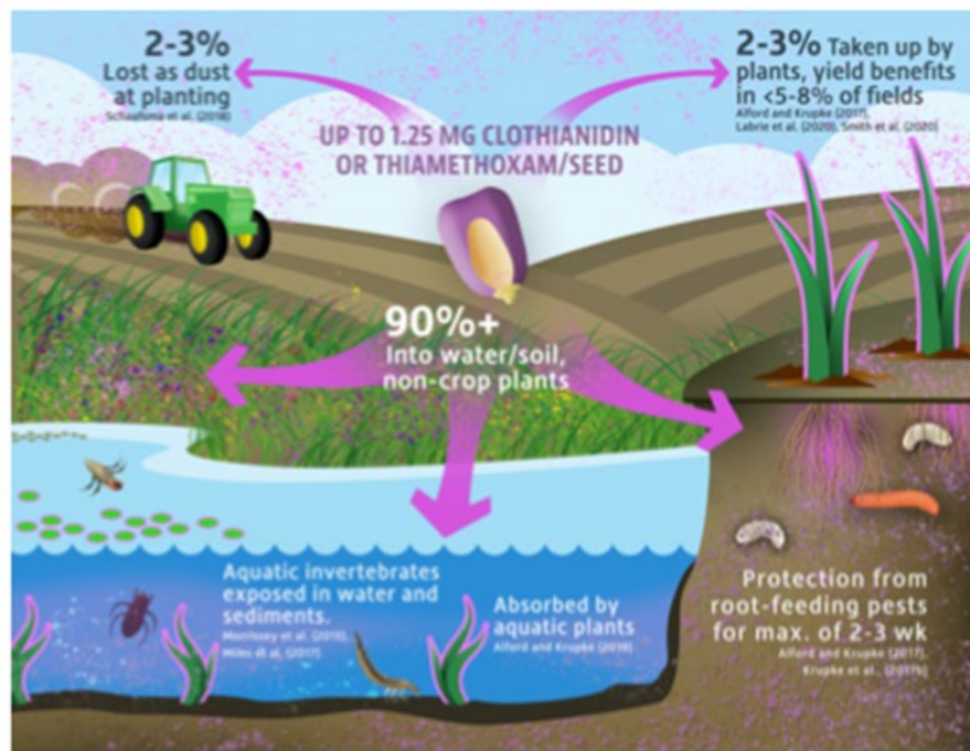
Schematic Representation of the Environmental Fate & Transport of Neonicotinoid Active Ingredients Applied to Crop Seeds 34
